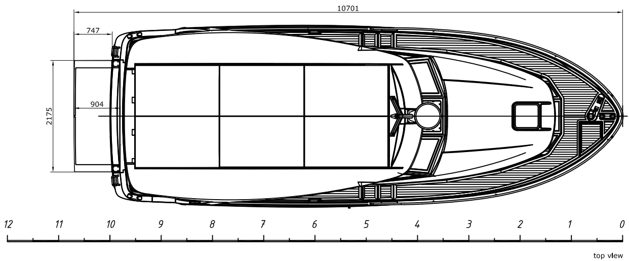
Greenline 33 - General dimensions
